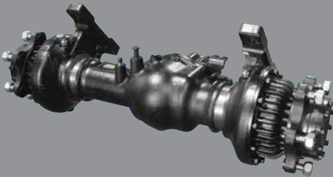
Highly Durable Split Type Drive Axle The bevel gear set and hub reduction axle smoothly delivers desired torque to the drive wheels.
